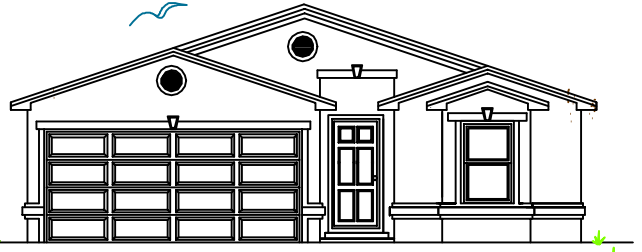
FRONT ELEVATION B
