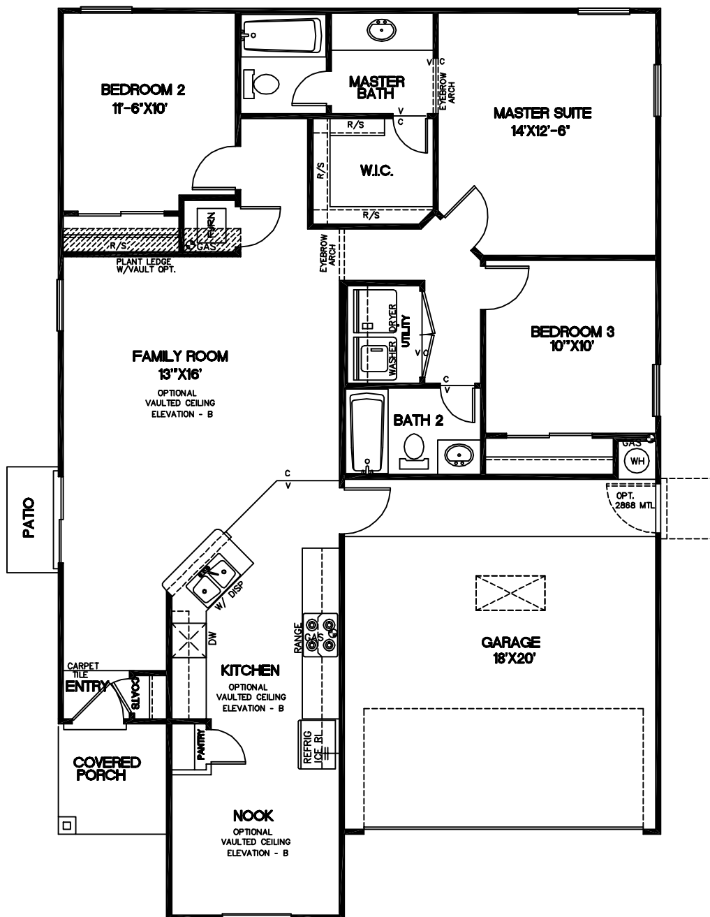
FLOORPLAN A & B
