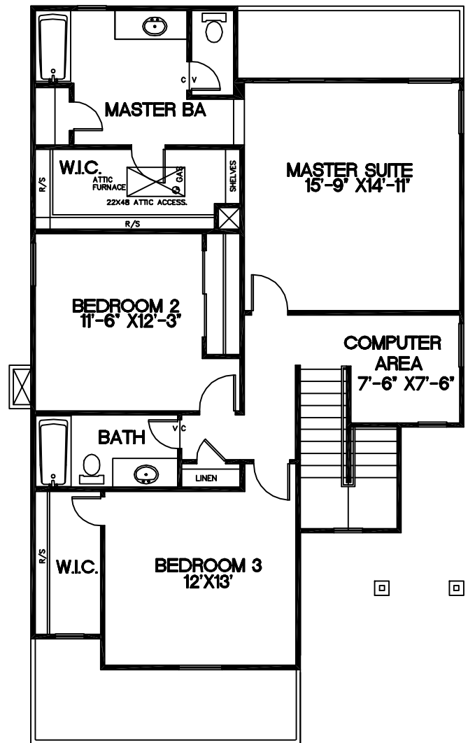
UPPER LEVEL A & B
