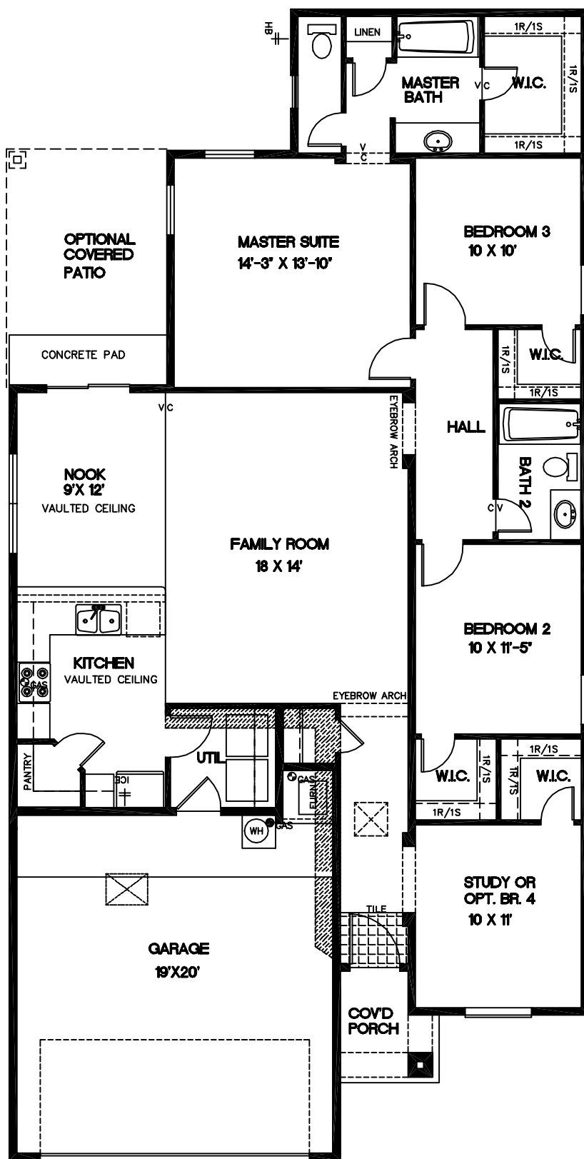
FLOORPLAN A & B
